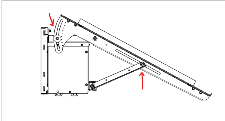
Figure 11. When the panel is adjusted to the desired angle, all 3/8 bolts should be tightened.
