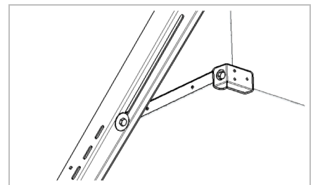
Figure 6. Note the placement of the wide washer.
