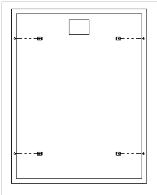
Figure 9. Install 1/4-20 clip nuts into the solar panel.
