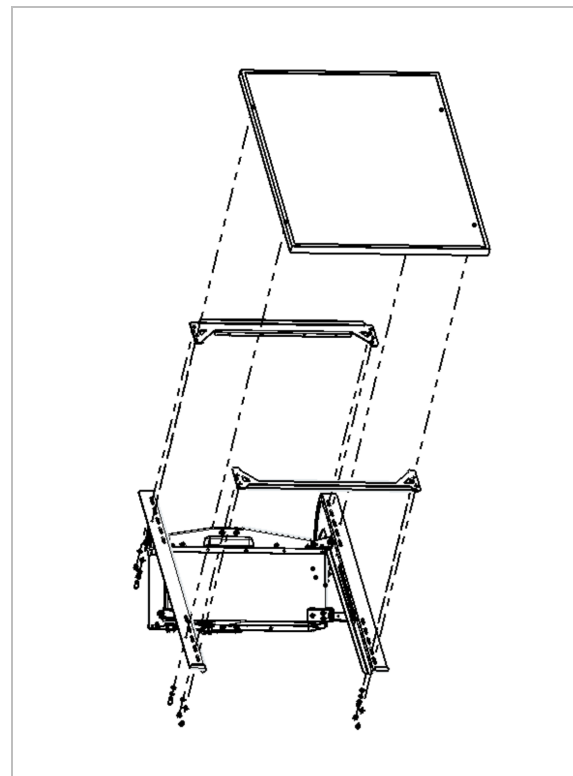
Figure 10. Attach the solar panel with the included hardware.
